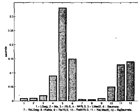
Figure 2. Computation time results for general and simplified methods with synthetic images.
