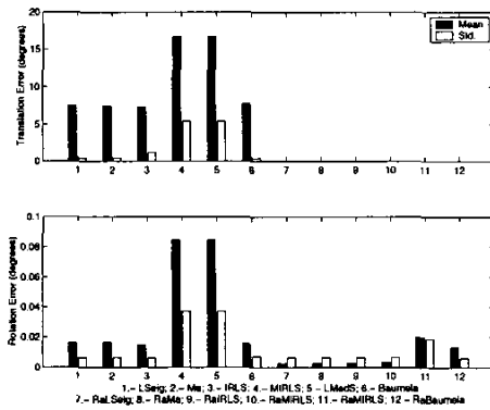
Figure 4. Results of general and simplified methods with real images.
