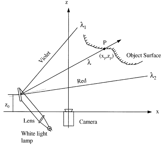
Fig. 18. The rainbow range pattern projected by Tajima et al. (62) made by a set of vertical slits which use the entire colour spectrum from violet to red.
