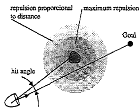
Fig. 4.1. Obstacle Avoidance principle.
