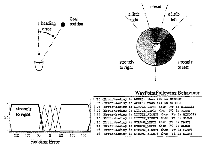
Fig. 4.1. WayPointFollowing behaviour based on the Heading error.
