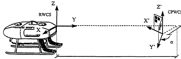
Figure 3.2. Relation between RWCS and CPWCS.
