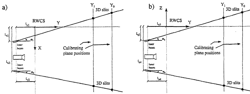
Figure 3.4. The geometrical relation between RWCS and laser beams. a) vertical laser beams, b) horizontal laser beams.
