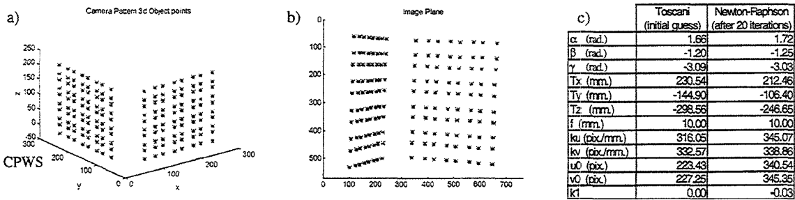
Figure 3.3. Camera Calibration : a) 3D points corresponding to the square vertexes of the pattern, b) 2D projective points on the image plane, and c) table shown camera parameters inferred by calibration.
