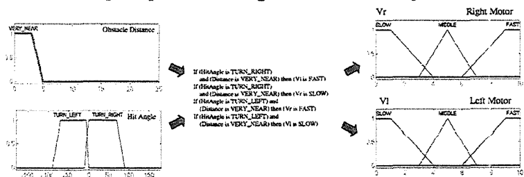
Fig. 3.4 Fuzzy implementation of the obstacle avoidance behaviour.
