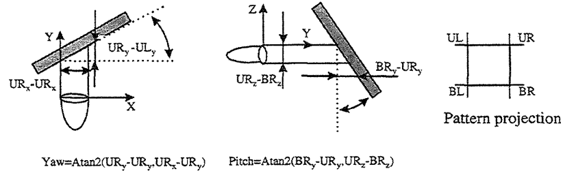
Fig. 4.5 Yaw and Pitch detection.
