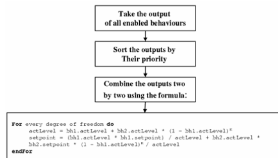
Figure. 8. Coordination algorithm.
